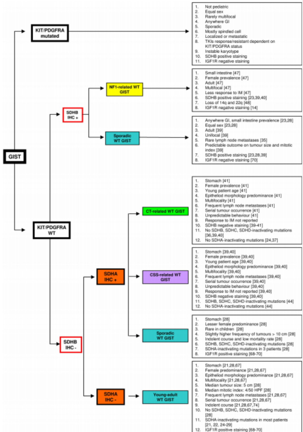
Figure 1 The molecular complexity of KIT/PDGFR \alpha WT GISTs.
